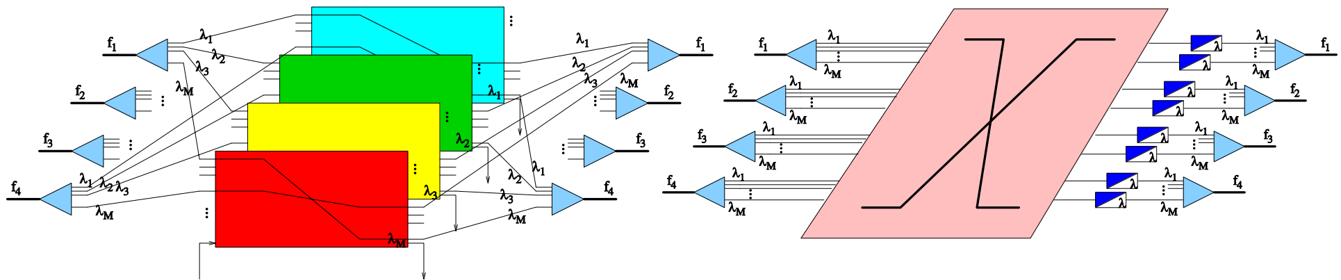
WT-OXC
